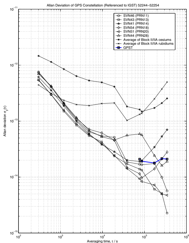
Figure 7. Allan deviation plot of each Block IIR satellite clock as well as a plot of the average Allan deviation of the Blocks II/IA cesium and II/IA rubidium satellites during December 2001. All clocks are referenced to IGST and no data editing has been applied.
